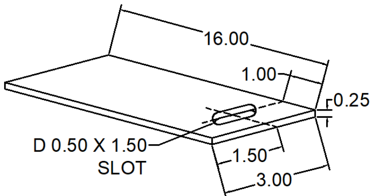
199 ANC-1603-199 WIND LOAD ANCHOR (MAIN CURTIAN WALL
