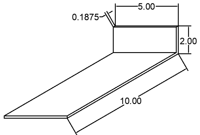
10 ANC-1025-10 ANCHOR CLIP
