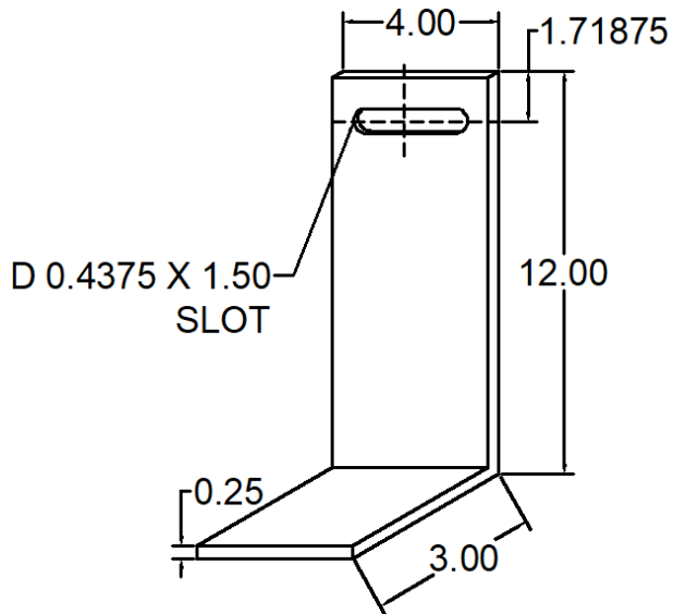
248 ANC-3124-248 WIND LOAD CLIP
