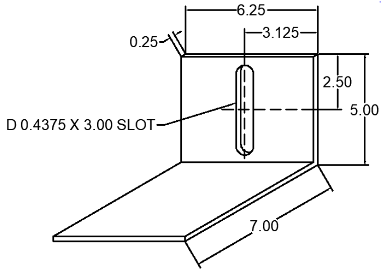
54 ANC-0705-54 WIND LOAD CLIP
