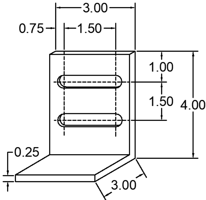
79 BMM-0000-M-79 WIND LOAD CLIP
