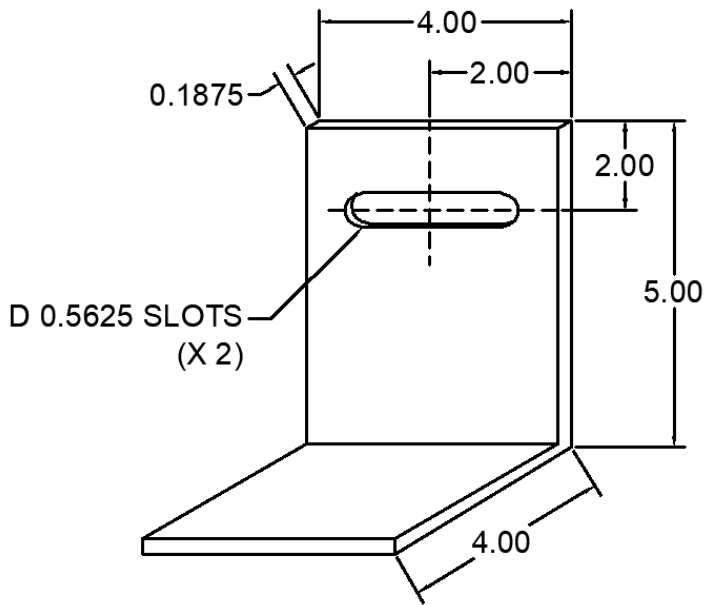
33 ANC-0445-33 WIND LOAD CLIP
