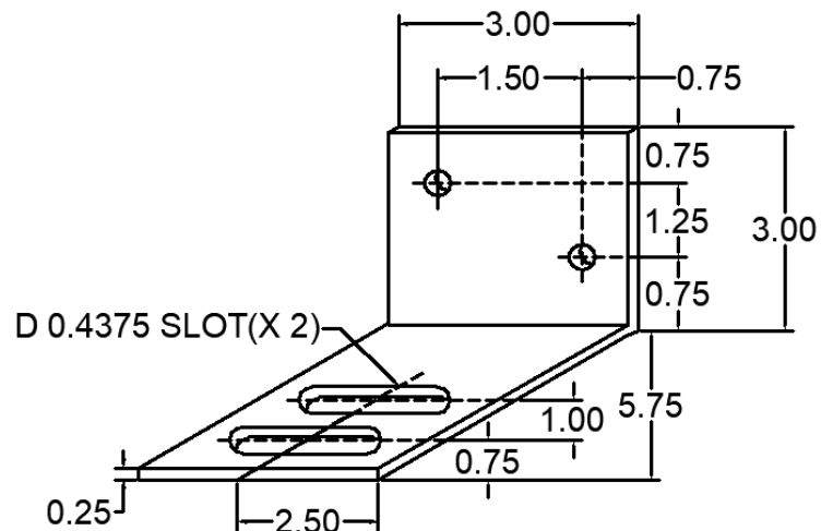
131 ANC-0303-5M1-131 WIND LOAD CLIP
