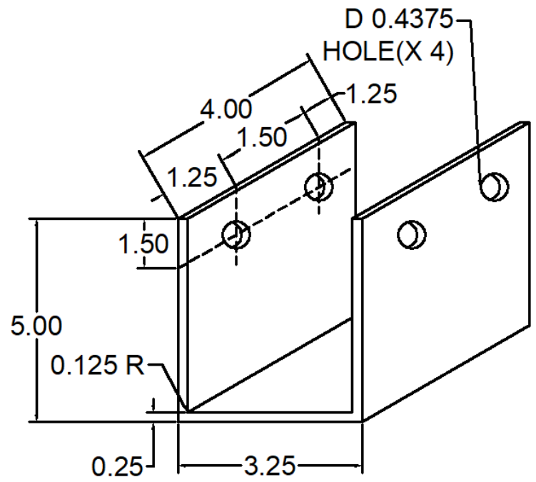
173 ANC-3255-DA-173 MULLIAN WRAP
