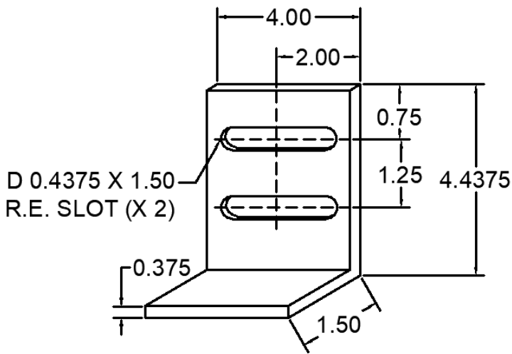
77 ANC-4715-77 WIND LOAD CLIP
