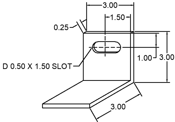
21 ANC-0001-21 WIND LOAD CLIP
