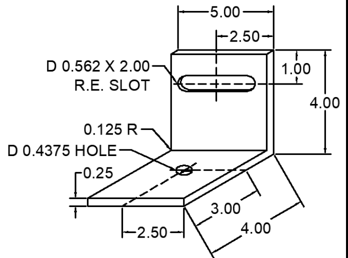
84 ANC-0404-WC-84 WIND LOAD CLIP
