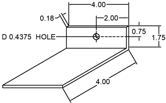
25 ANC-0404-1M-25 DEAD LOAD CLIP
