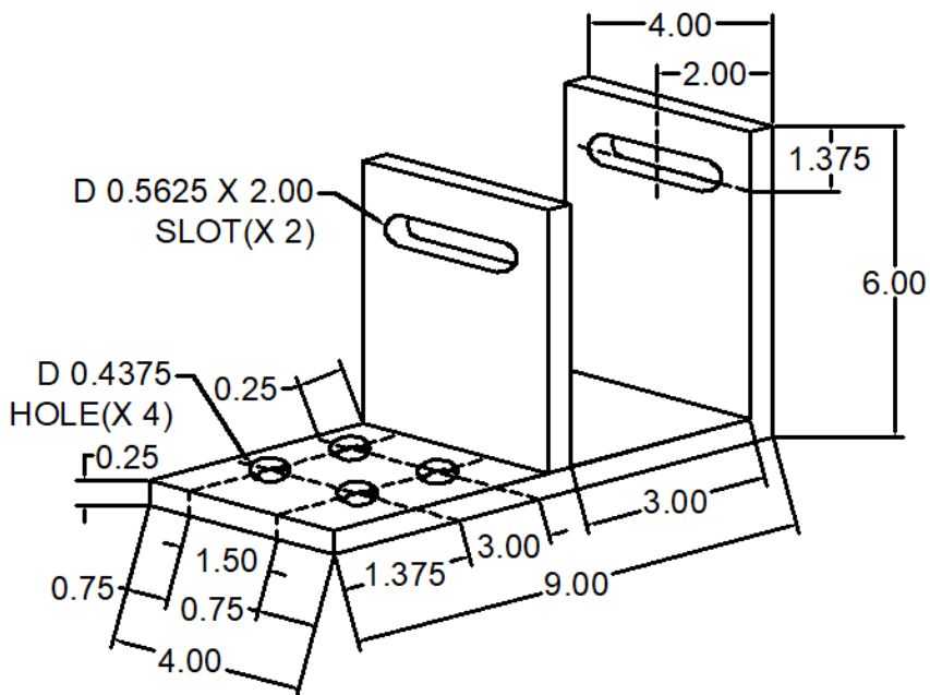
209 ANC-0904-6-209 SIDE MOUNT/DEAD LOAD
