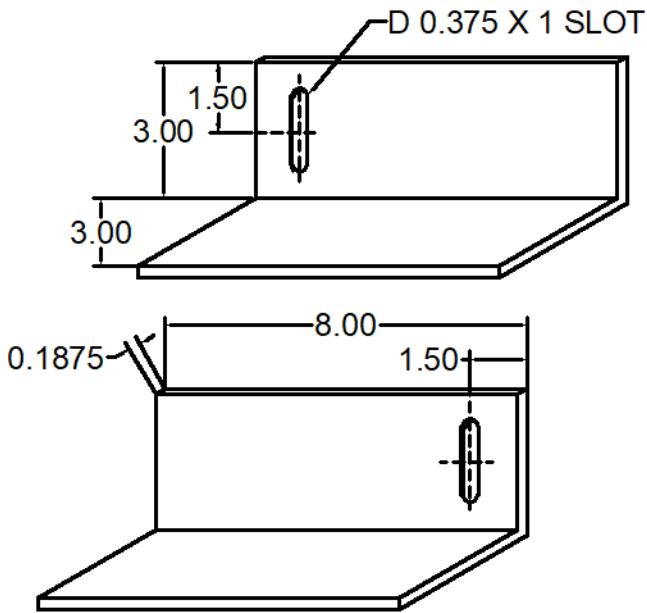
53 ANC-0303-8-53 WIND LOAD CLIP
