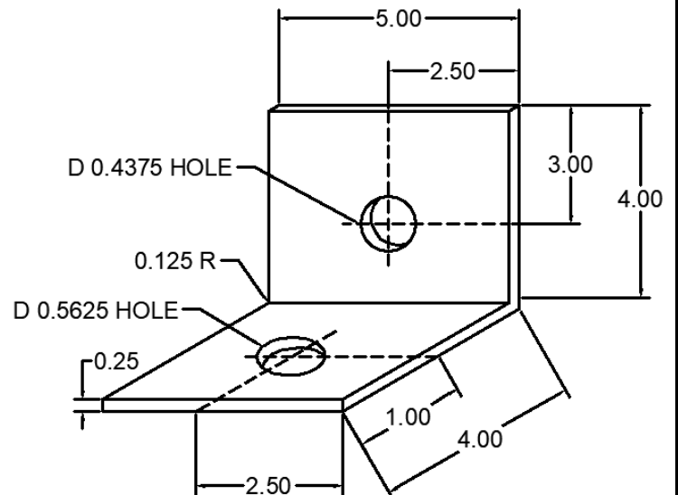
88 ANC-0404-DC-88 DEAD LOAD CLIP
