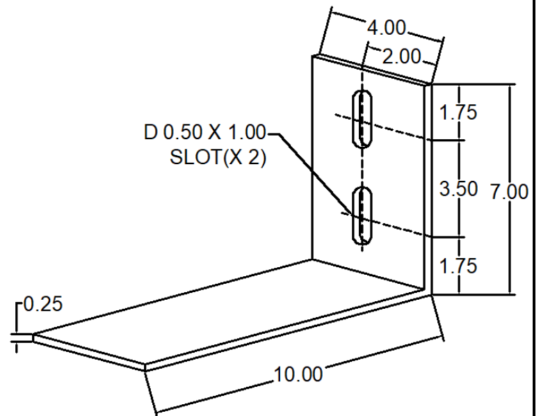
251 ANC-7104-251 WIND LOAD CLIP
