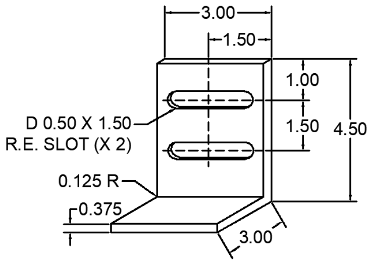
81 ANC-0304-M-81 WIND LOAD CLIP
