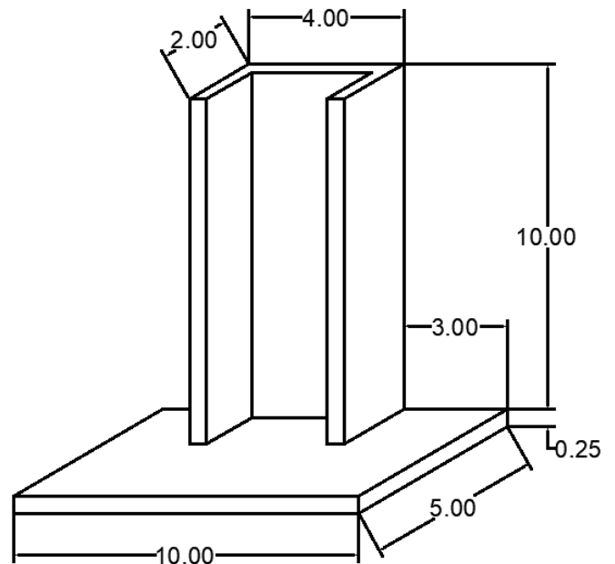
213 ANC-0510-AC-213 SLIP MULLIAN ATTACHMENT CLIP
