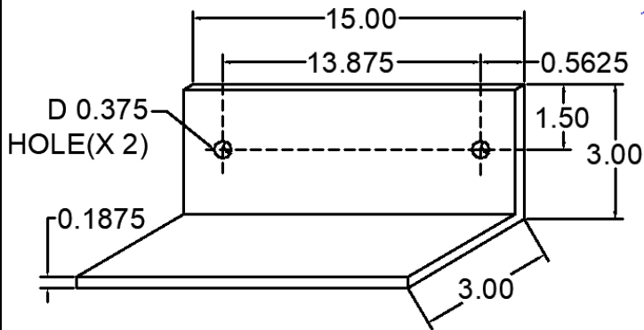
108 ANC-0303-15-108 FLOOR ANCHOR
