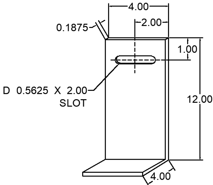
67 ANC-0412-WL-67 WIND LOAD CLIP
