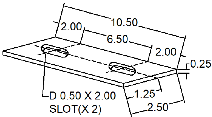
203 ANC-0210-9-203 WIND LOAD GIRT ANCHOR
