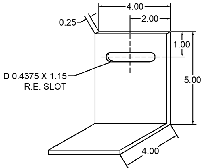
35 ANC-0305-C-35 WIND LOAD CLIP
