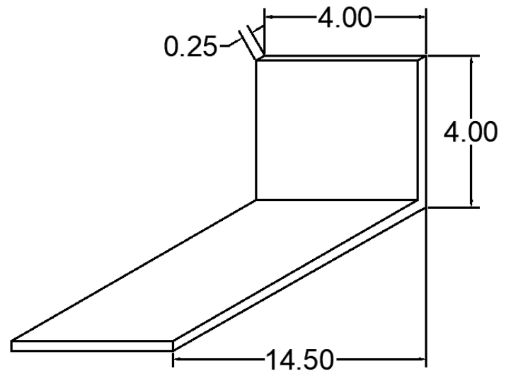
16 ANC-3144(W-1)-16 ANCHOR CLIP
