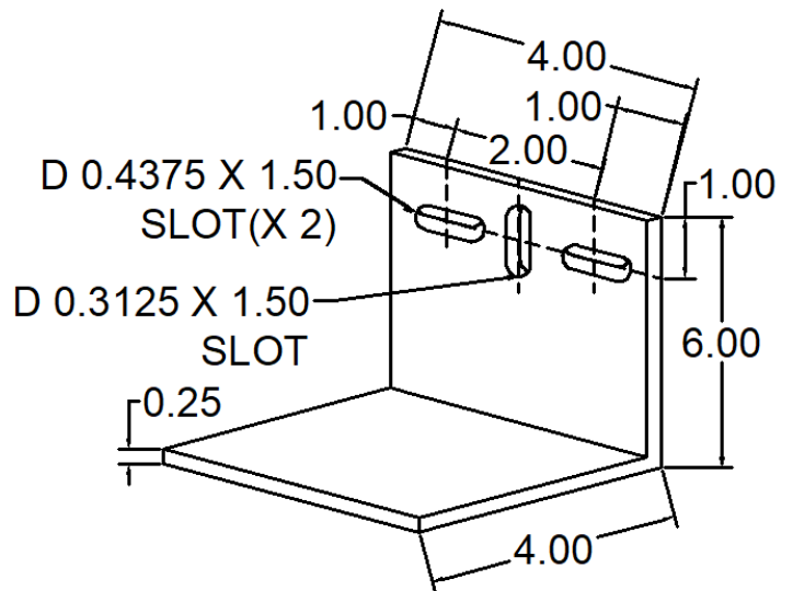
318 WLA-5595-318 WIND LOAD CLIP
