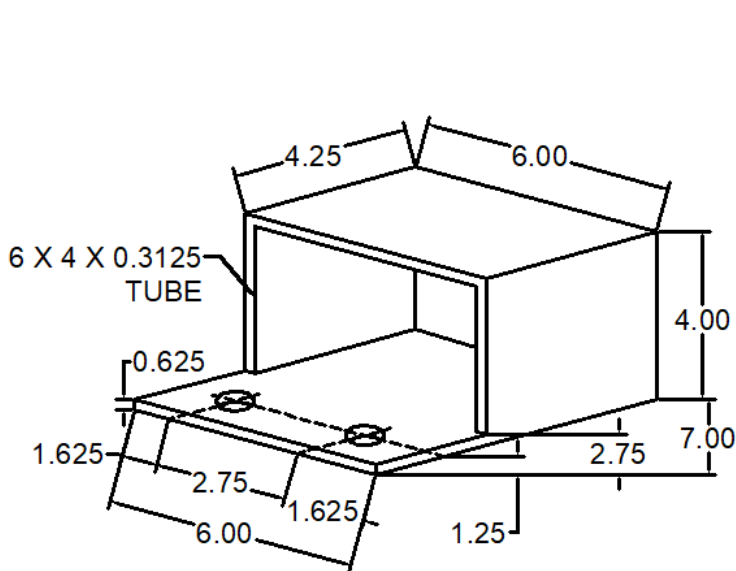
282 TUB-4607-282 DEAD LOAD ANCHOR WELD TO BEAM
