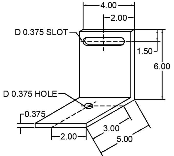
97 ANC-0506-CW-97 WIND LOAD CLIP
