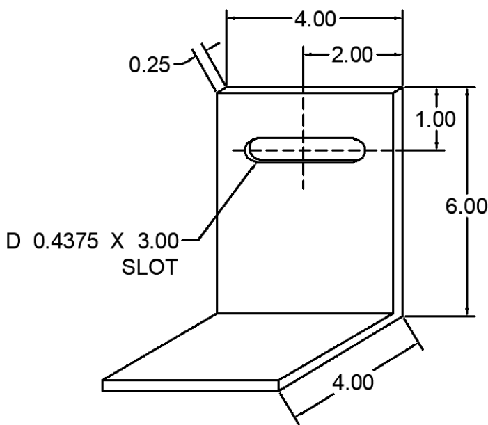
41 ANC-0604-4-41 WIND LOAD CLIP
