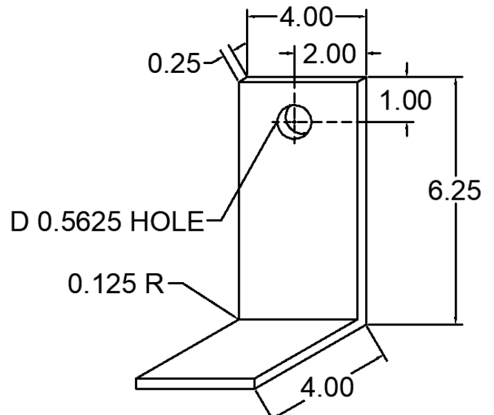
52 ANC-0406-4DL-52 DEAD LOAD CLIP
