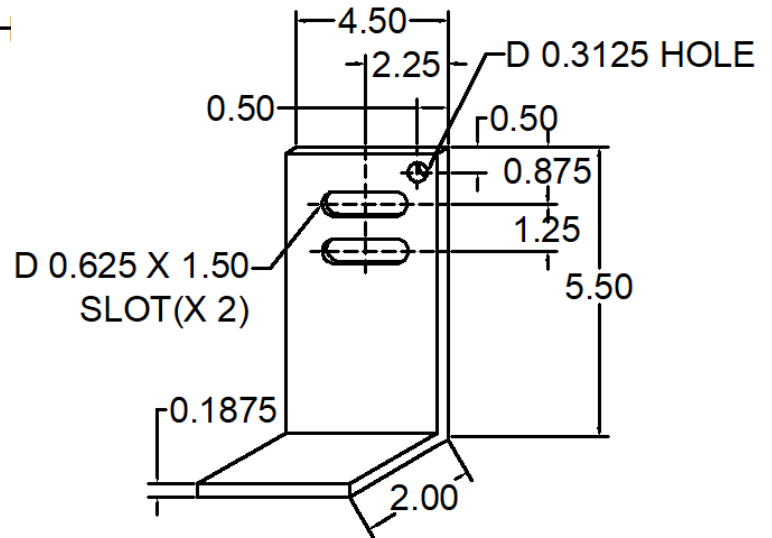
322 WLA-4565-322 WIND LOAD CLIP
