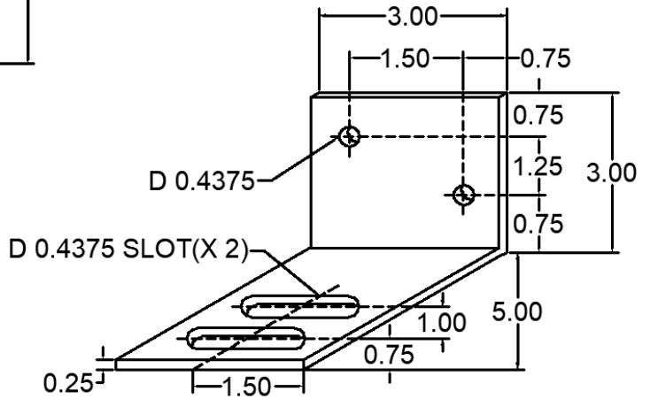
140 ANC-0303-5M3-140 WIND LOAD CLIP
