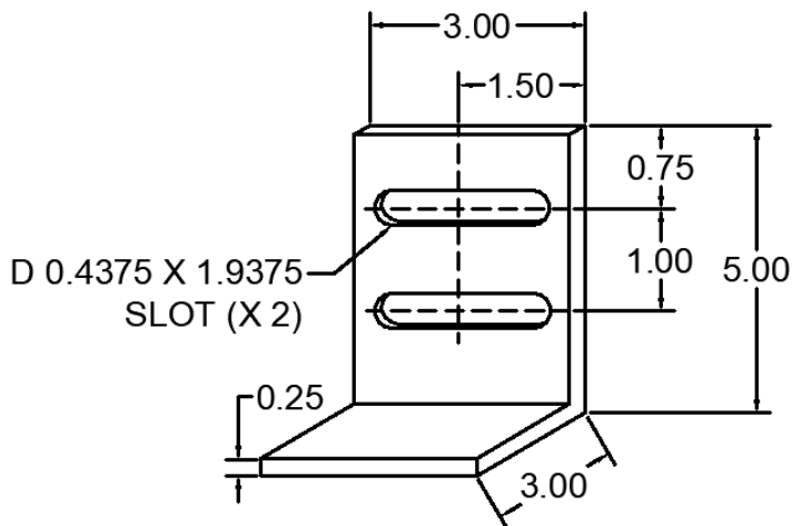
83 ANC-0303-5M-83 WIND LOAD CLIP
