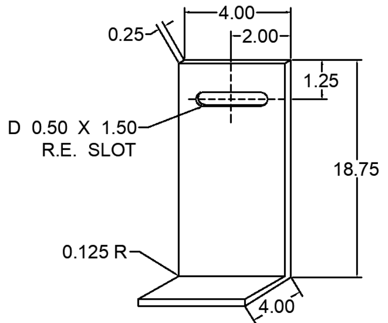
64 ANC-0404-18WC-64 WIND LOAD CLIP
