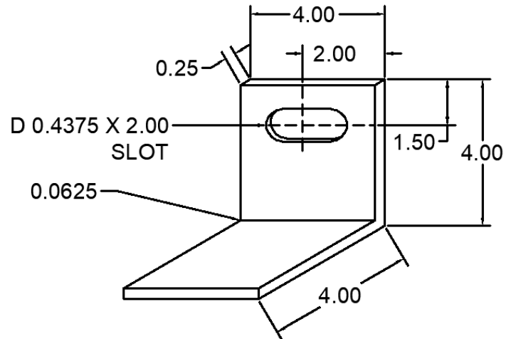
30 ANC-0404-4M-30 WIND LOAD CLIP
