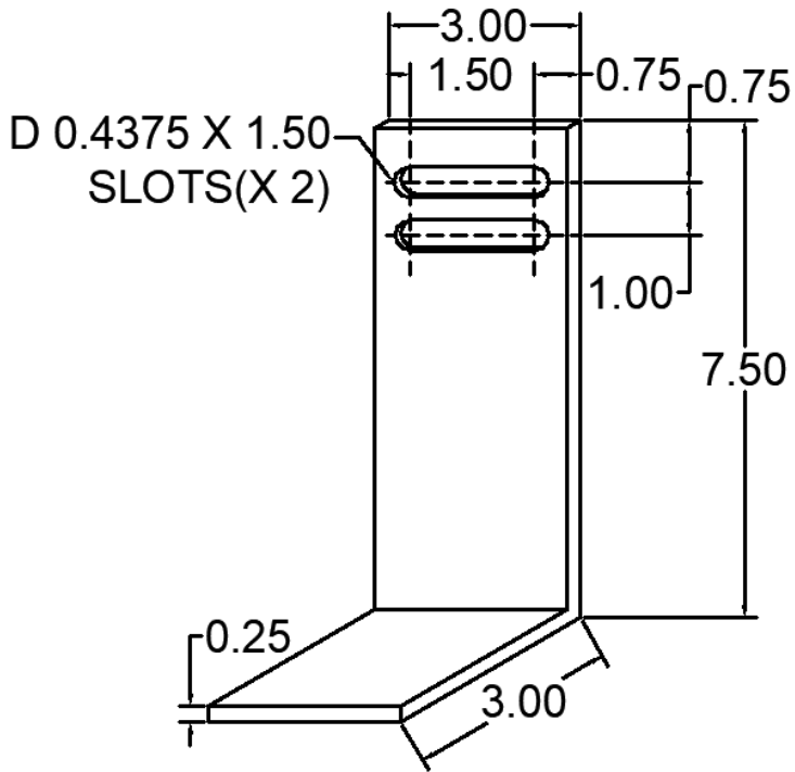
100 ANC-0307-M-100 WIND LOAD CLIP
