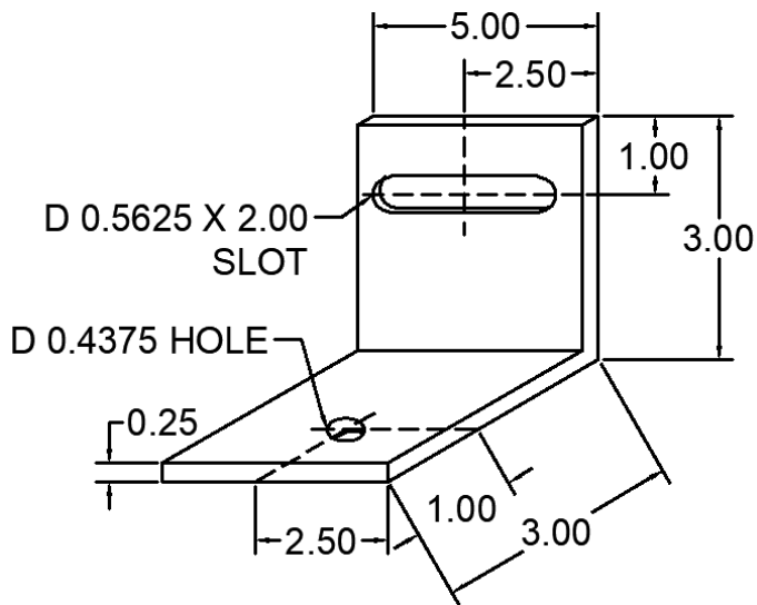
85 ANC-0404-WG-85 WIND LOAD CLIP
