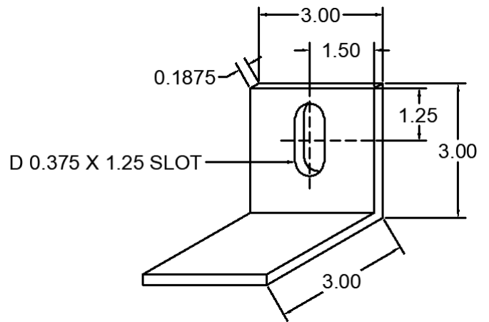
22 ANC-0303-3M-22 WIND LOAD CLIP
