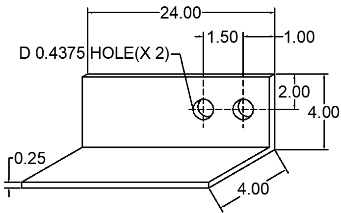
104 ANC-0424-104 DEAD LOAD CLIP
