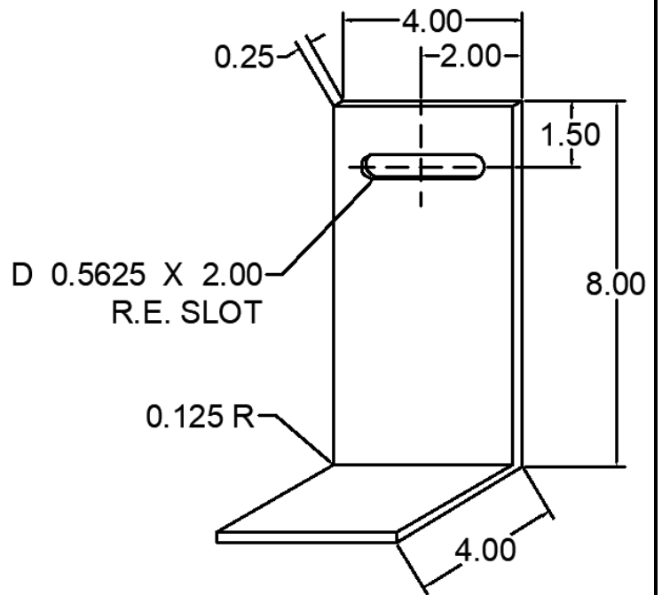
58 ANC-0408-58 WIND LOAD CLIP
