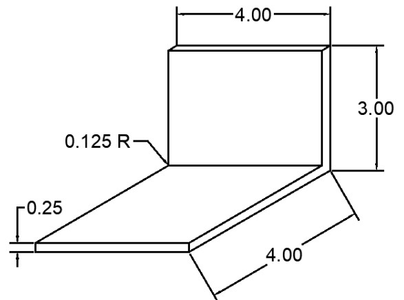
4 ANC-3404-4 ANCHOR CLIP
