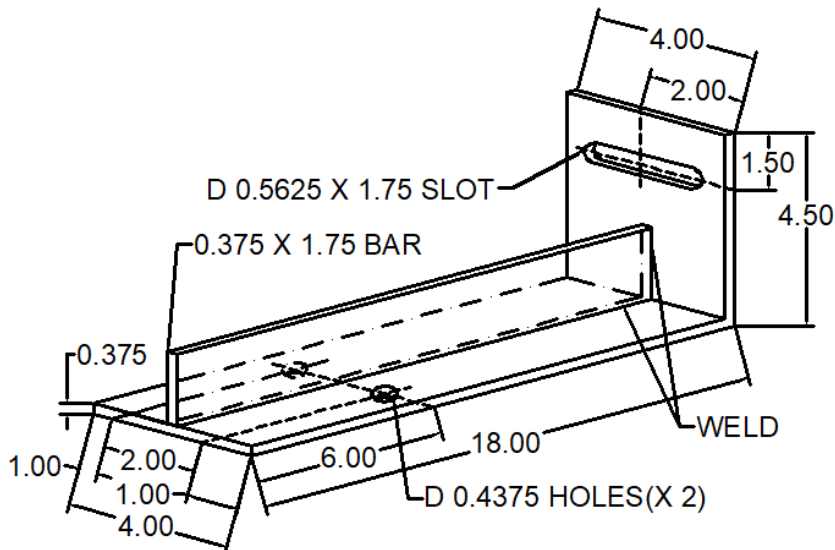
333 ANC-4535-333 CANTILEVER WIND LOAD ARM BRACKET ANCHOR
