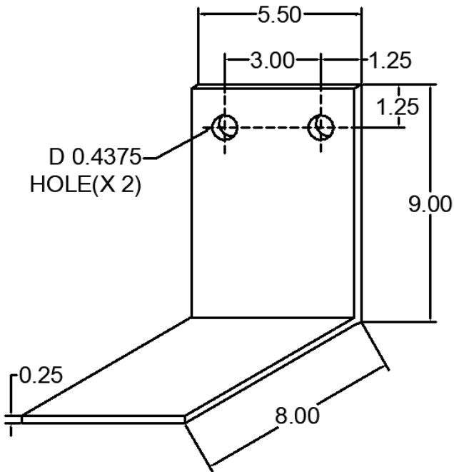
112 ANC-0809-5-112 DEAD LOAD CLIP
