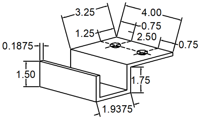
300 ANC-4155-300 FORMED HEAD ANCHOR
