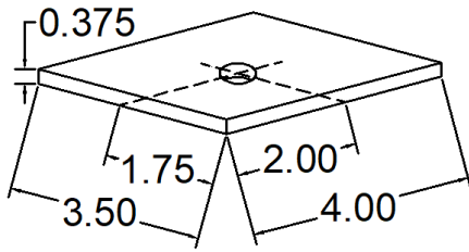
284 PLA-4035-284 SHIM PLATE
