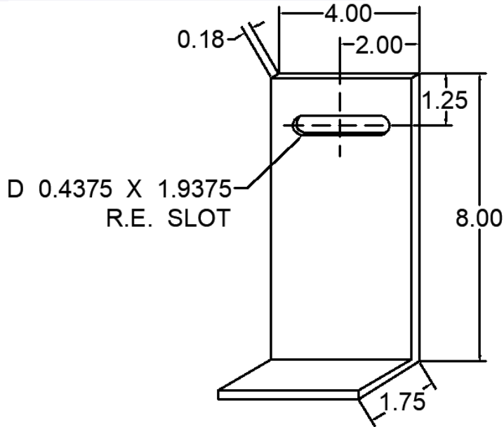
57 ANC-0408-M-57 WIND LOAD CLIP
