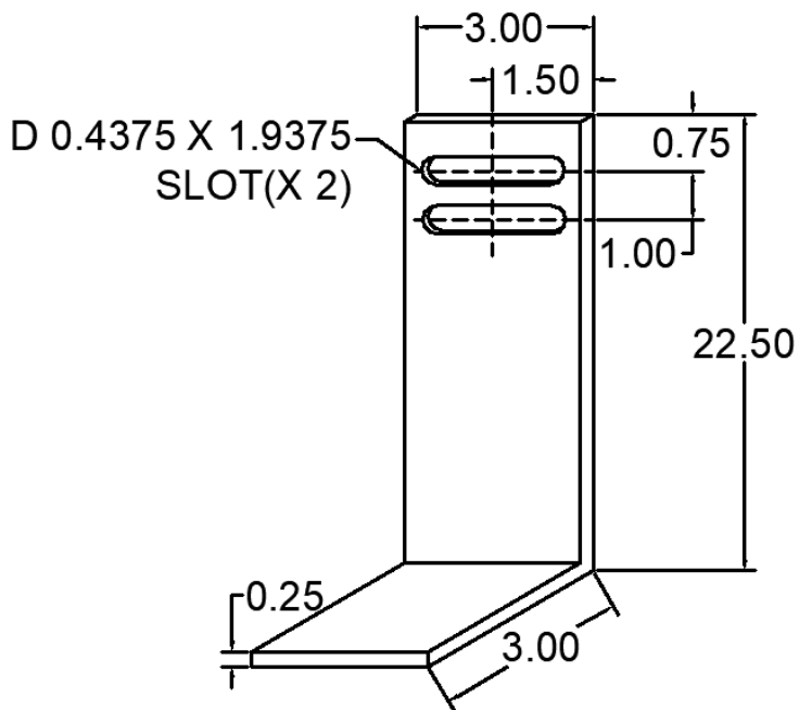
102 ANC-0303-22-102 WIND LOAD CLIP
