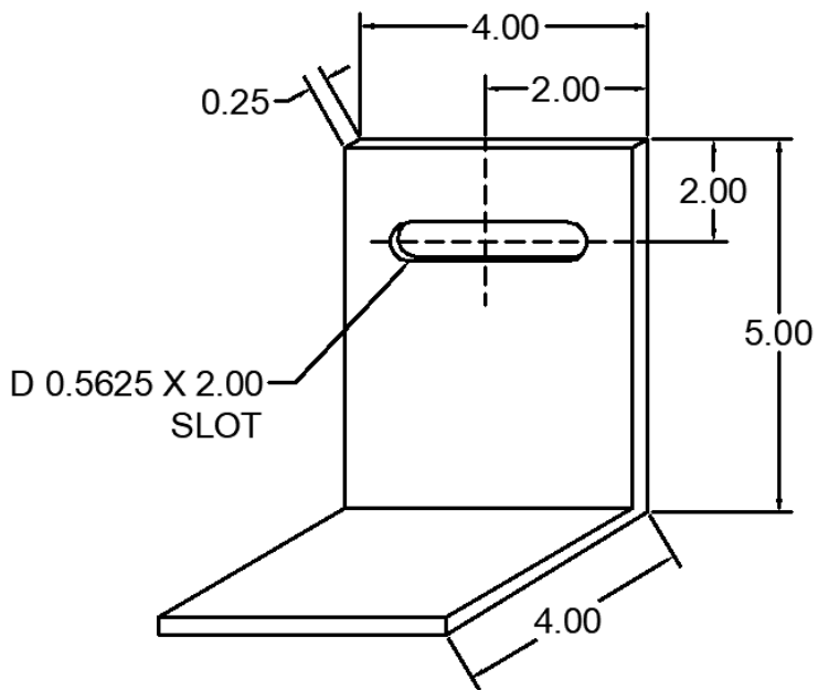
37 ANC-0405-4-37 WIND LOAD CLIP
