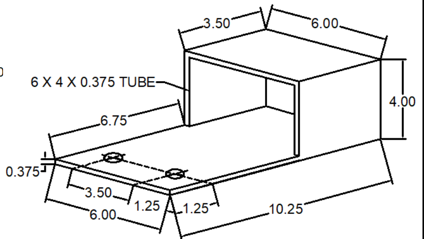
291 TUB-6410-291 DEAD LOAD ANCHOR WELD TO COLUMN/BEAM
