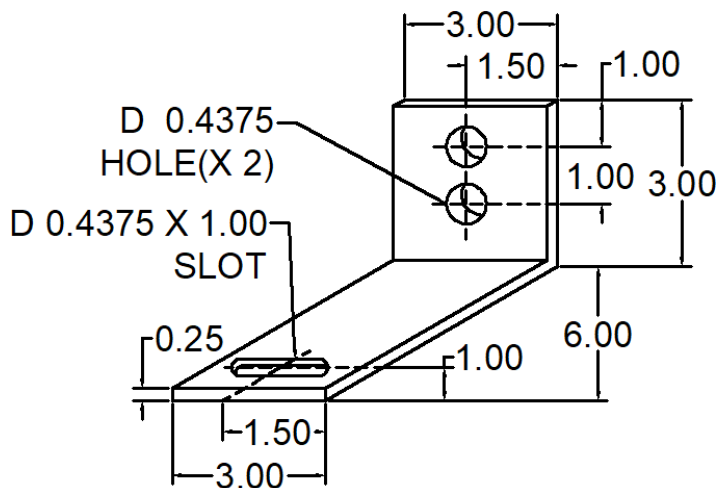
258 ANC-6303-258 WIND LOAD CLIP
