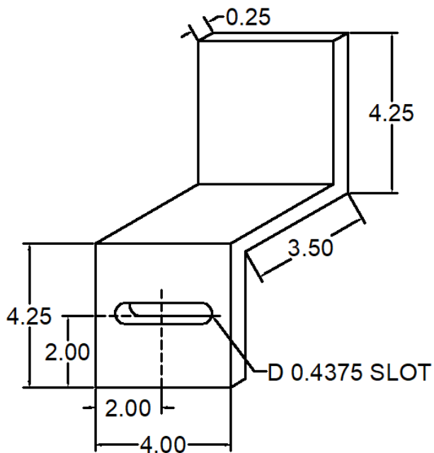
181 ANC-0404-WCZ-181 WIND LOAD HANGER
