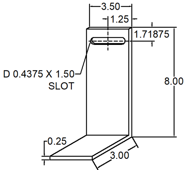
240 ANC-3804-240 WIND LOAD CLIP
