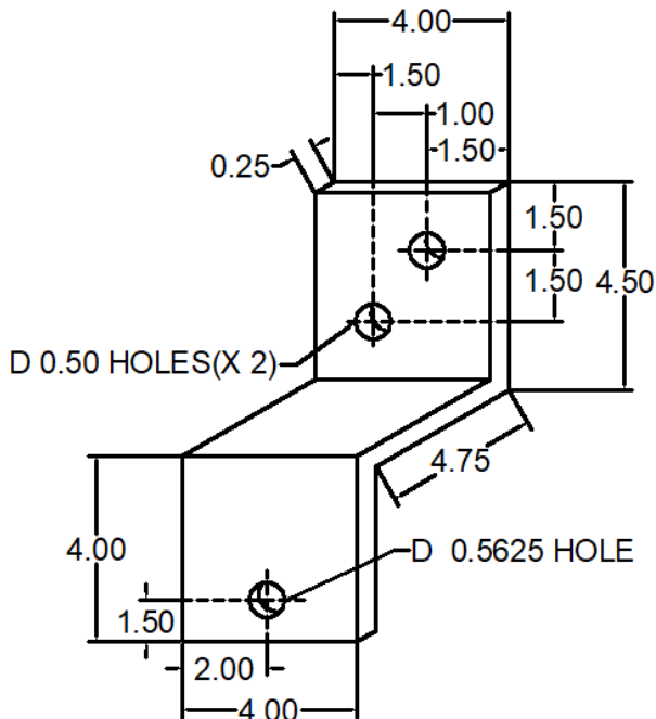
189 ANC-0404-DLZ-189 “Z” SHAPE DEAD LOAD CLIP
