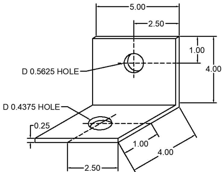
87 ANC-0404-G-87 DEAD LOAD CLIP
