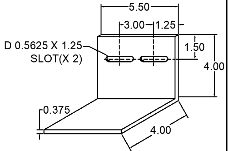
94 ANC-0405-5M-94 WIND LOAD CLIP
