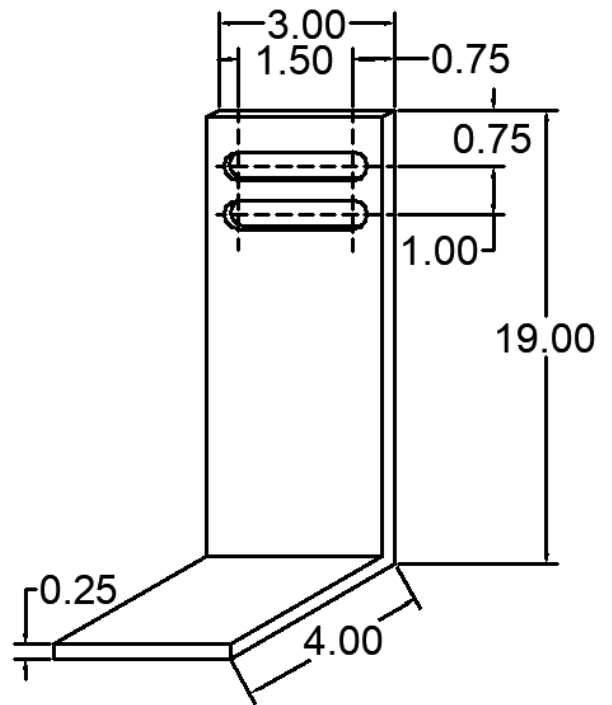
101 ANC-0304-19-101 WIND LOAD CLIP
