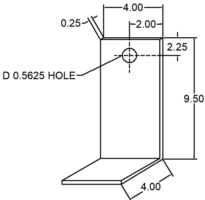
69 ANC-0404-9DL-69 DEAD LOAD CLIP
