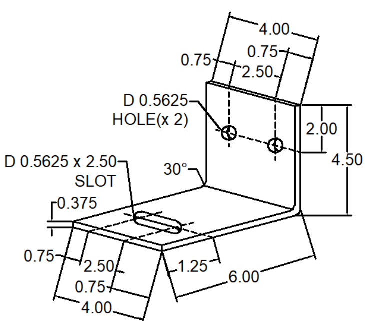
296 ANC-4564-296 WIND LOAD CLIP
