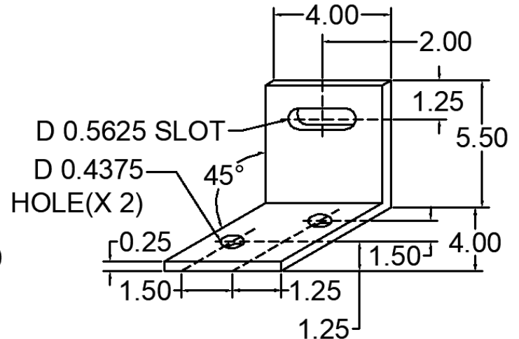
121 ANC-0405-4WL-121 45° DEGREE WIND LOAD
