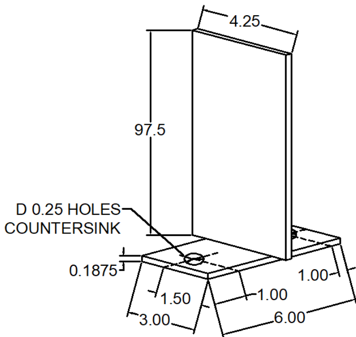
211 ANC-0095-211 "T" MULLIAN BASE ANCHOR
