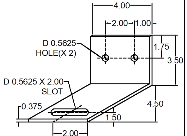
324 ANC-4535-324 WIND LOAD CLIP
