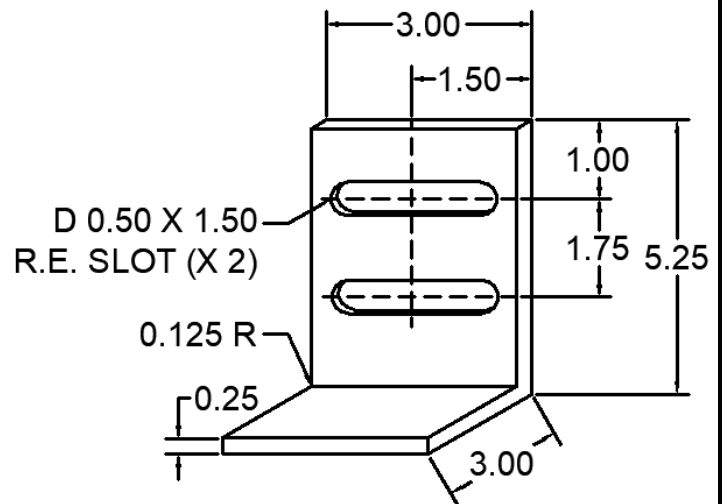
82 ANC-0304-WM-82 WIND LOAD CLIP
