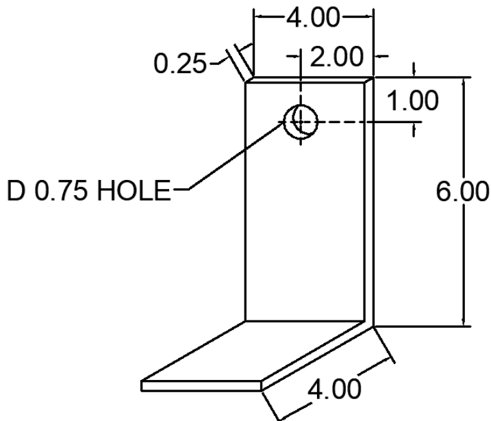
51 ANC-0604-4M-51 DEAD LOAD CLIP
