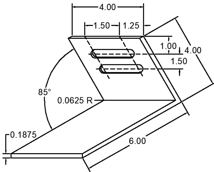
93 ANC-0604-C-93 WIND LOAD CLIP
