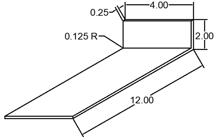
14 ANC-0412-14 ANCHOR CLIP
