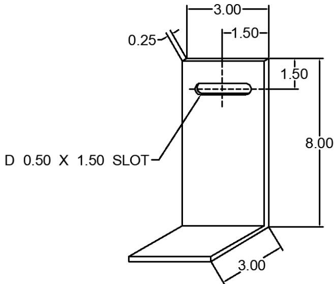
55 ANC-0308-55 WIND LOAD CLIP
