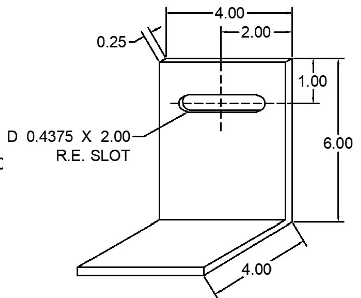
38 ANC-0405-M-38 DEAD LOAD CLIP
