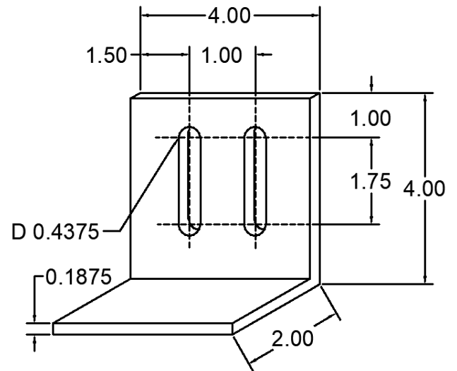
78 ANC-0404-2-78 WIND LOAD CLIP
