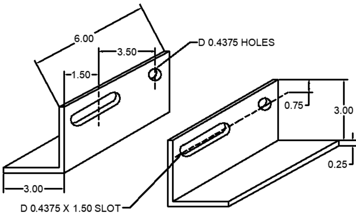
95 ANC-0303-6M-95 Entry Frame Jumbuck
