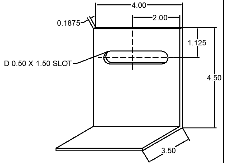
26 ANC-0304-WC-26 WIND LOAD CLIP
