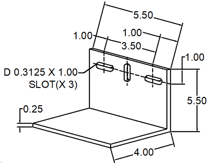
318 WLA-5595-318 WIND LOAD CLIP
