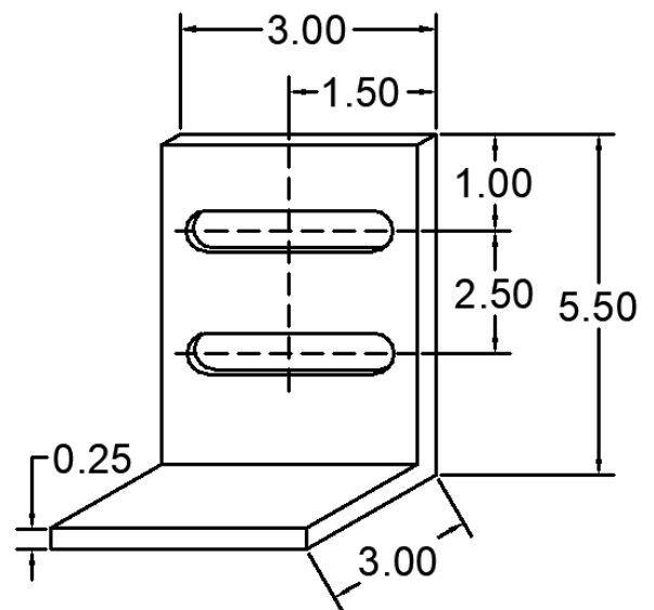
80 ANC-0305-80 WIND LOAD CLIP
