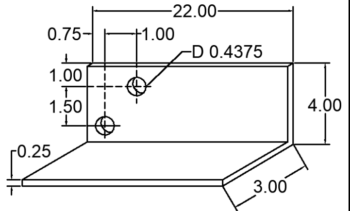
105 ANC-0403-22-105 DEAD LOAD CLIP
