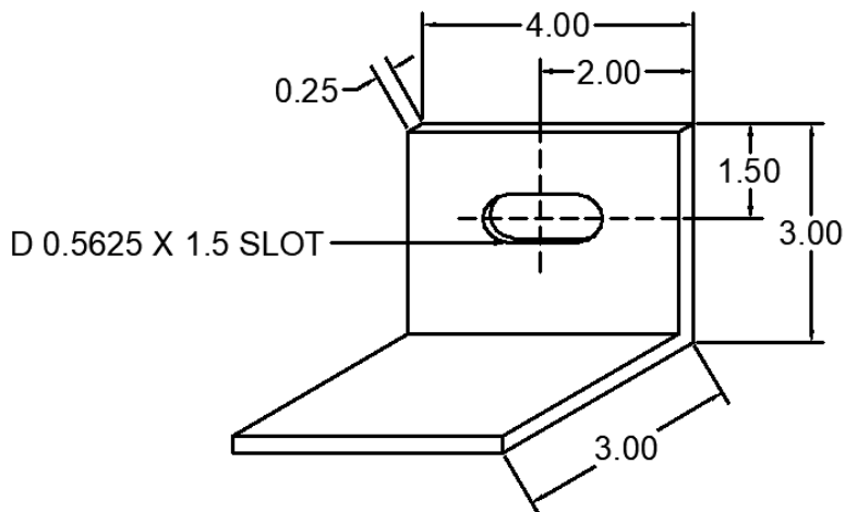
23 ANC-0304-23 WIND LOAD CLIP
