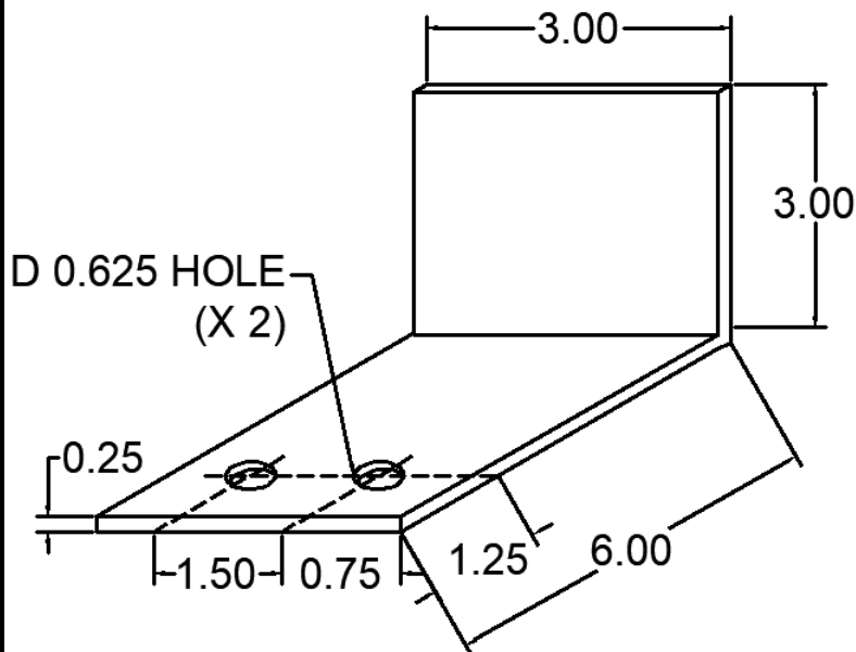
91 ANC-0604-C-93 DEAD LOAD CLIP
