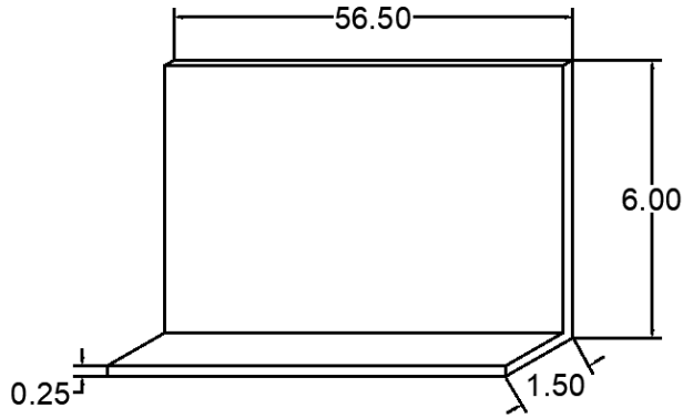
17 ANC-0604-17 ANCHOR CLIP
