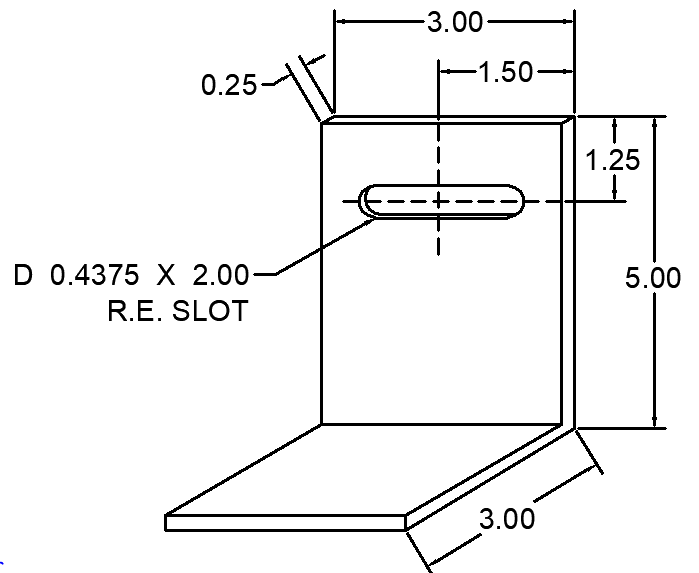
36 ANC-0305-WC-36 WIND LOAD CLIP
