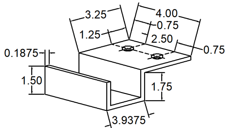
301 ANC-4173-301 FORMED HEAD ANCHOR
