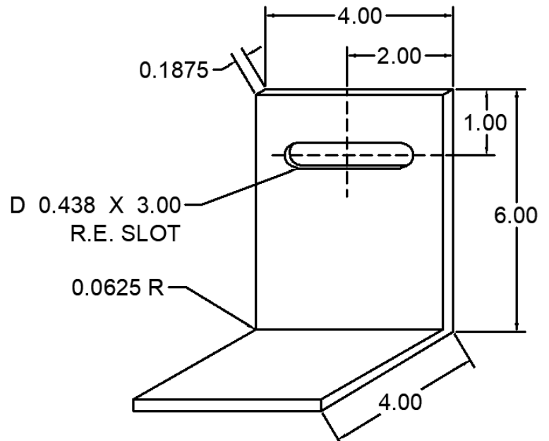
42 ANC-0404-6-42 WIND LOAD CLIP
