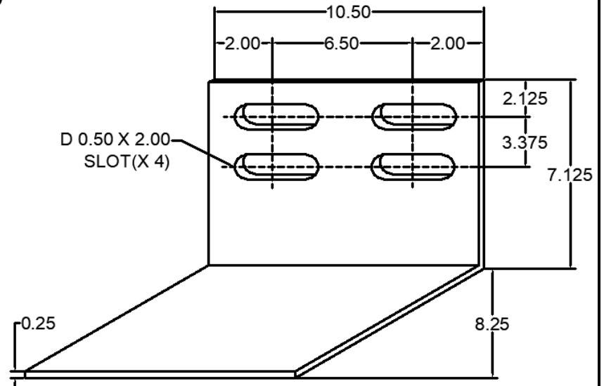
137 ANC-8271-137 WIND LOAD CLIP
