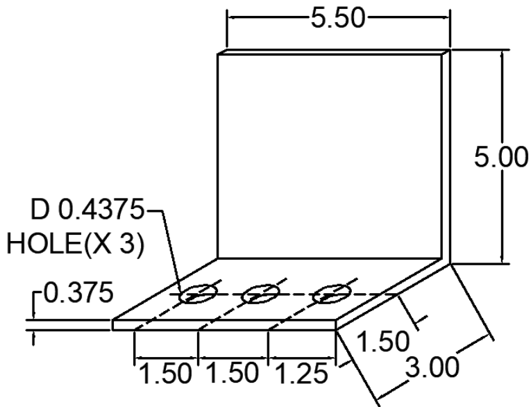
112 ANC-0809-5-112 DEAD LOAD CLIP
