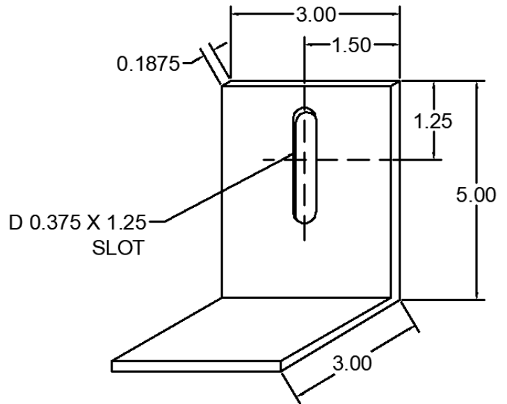
34 ANC-0303-5M6-34 WIND LOAD CLIP
