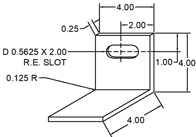
31 ANC-0303-4M-31 WIND LOAD CLIP
