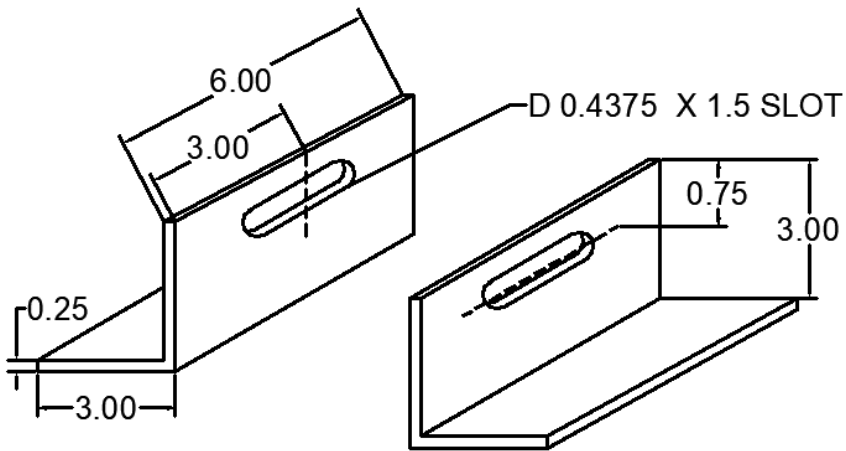
45 ANC-0303-6M-45 WIND LOAD CLIP
