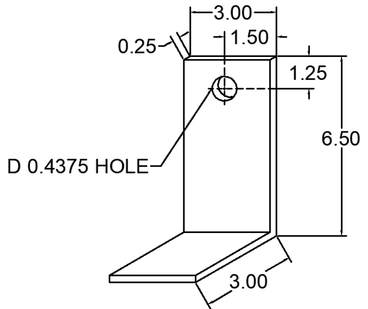
50 ANC-0306-DC-50 DEAD LOAD CLIP
