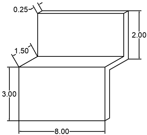
179A ANC-0203-Z-179A ANGLE "Z" CLIP
