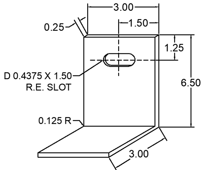
48 ANC-0306-WC-48 WIND LOAD CLIP
