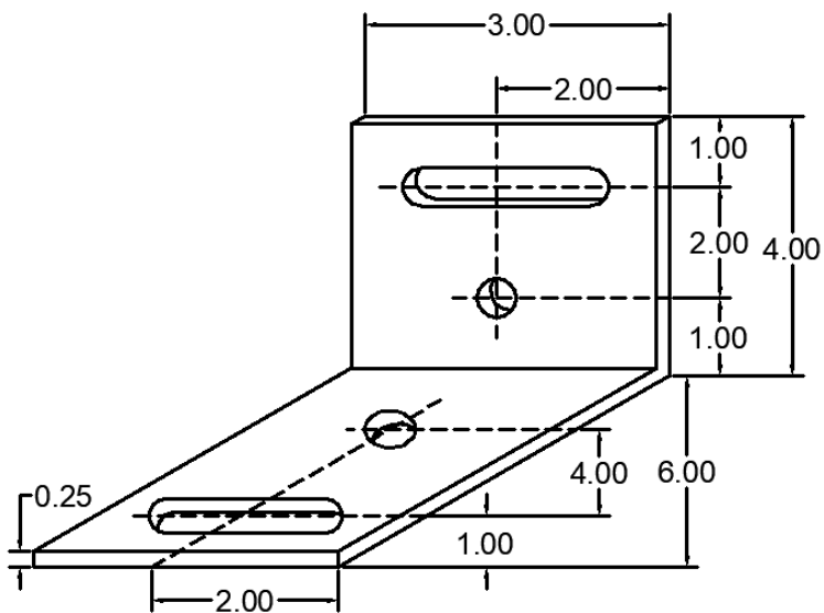
138 ANC-0406-4M-138 CURTAIN WALL WIND LOAD CLIP
