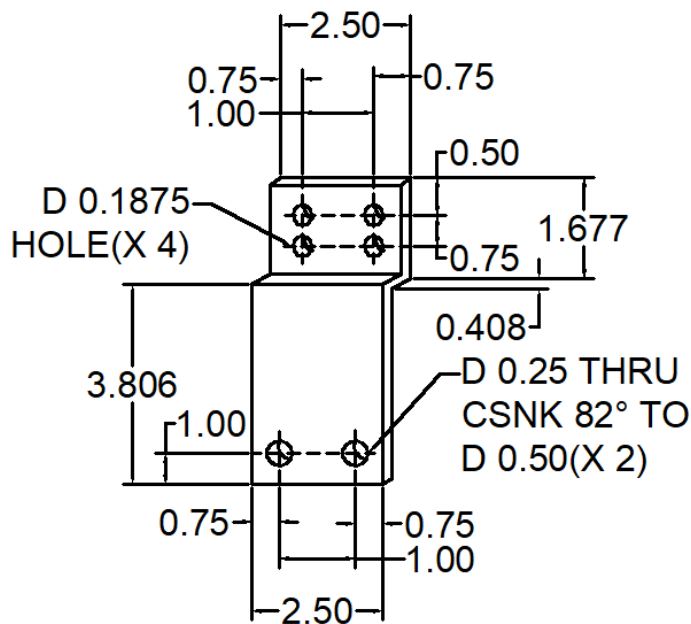
187 ANC-0205-A-187 ALUMINUM SPLICE OFFSET DEAD LOAD
