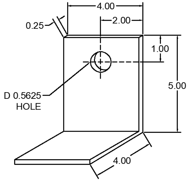
38 ANC-0405-M-38 DEAD LOAD CLIP
