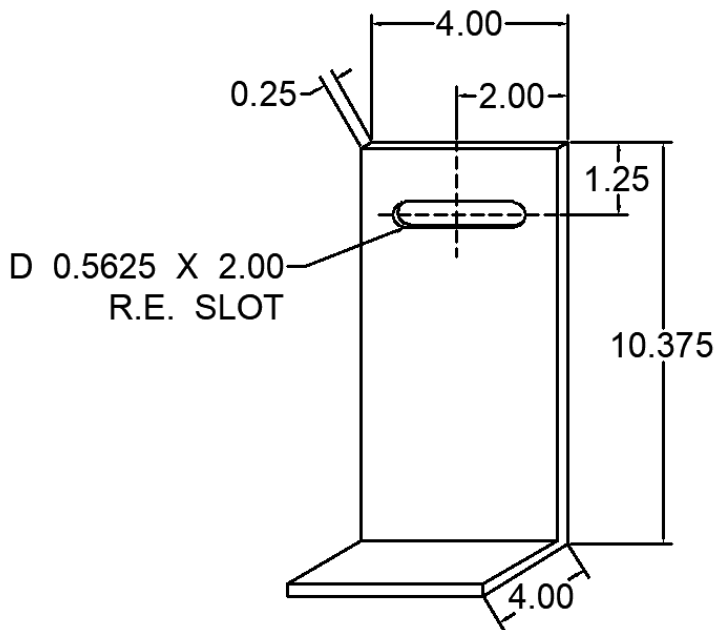
65 ANC-0410-WA-65 WIND LOAD CLIP
