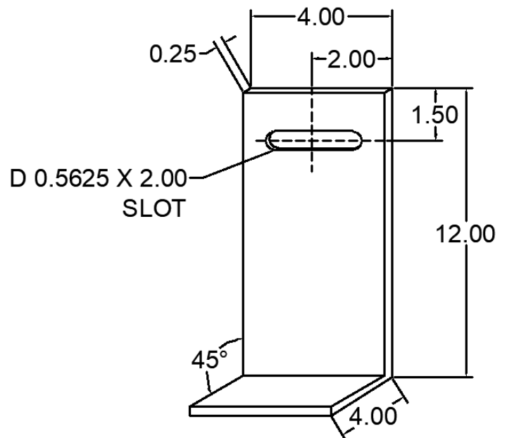
72 ANC-0404-12WL-72 WIND LOAD CLIP
