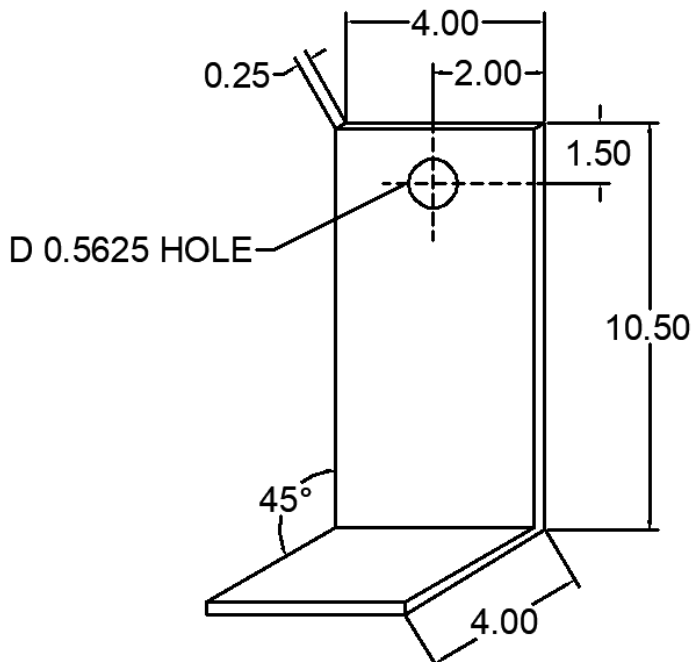
71 ANC-0404-12DL-71 DEAD LOAD CLIP
