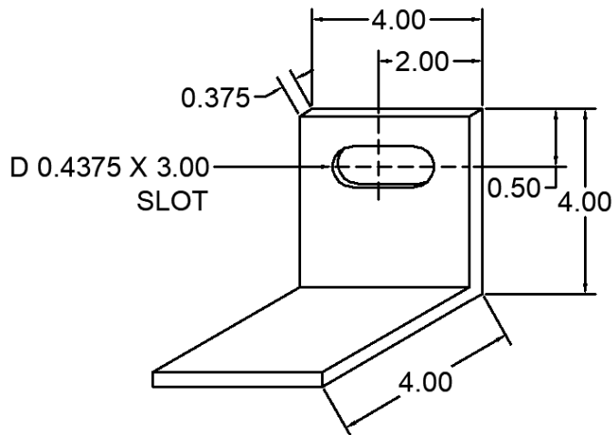
29 ANC-0404-4-29 WIND LOAD CLIP
