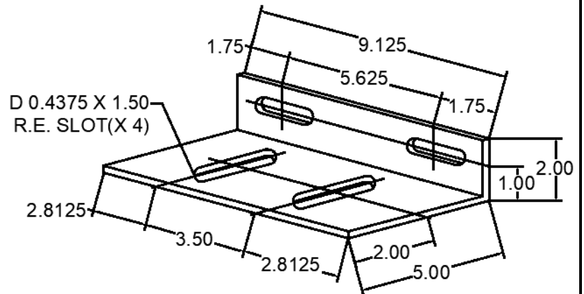
221 ANC-2592-221 WIND LOAD CLIP
