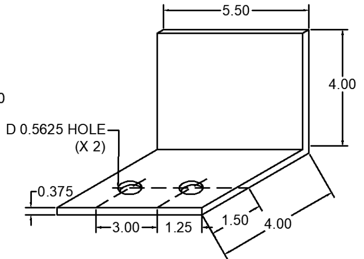
90 ANC-0404-5-90 DEAD LOAD CLIP
