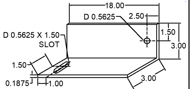
109 ANC-0303-18(LH/RH)-109 WIND LOAD ANCHOR
