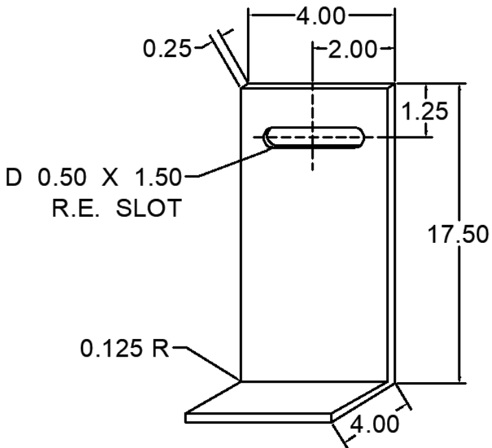
63 ANC-0404-17WC-63 WIND LOAD CLIP
