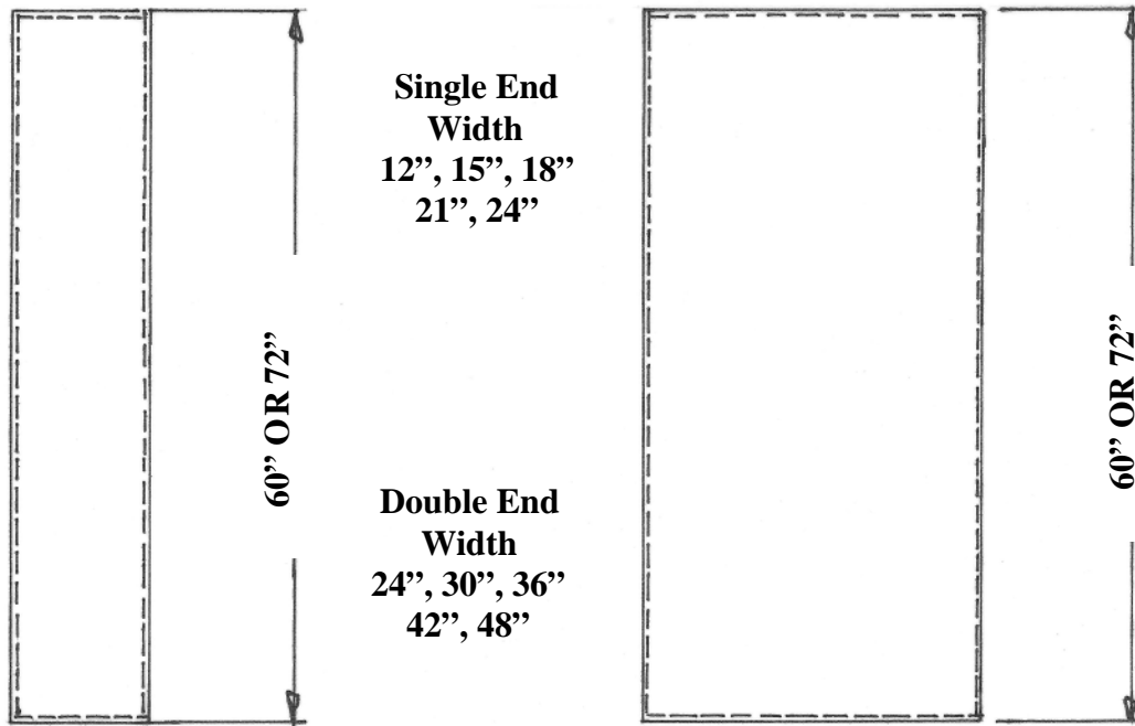
Single End
