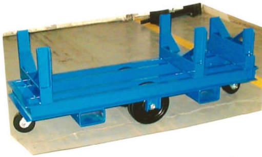
BTC-0096 Bar Cradle Truck Modified for Rocket Assembly w/fork tubes
