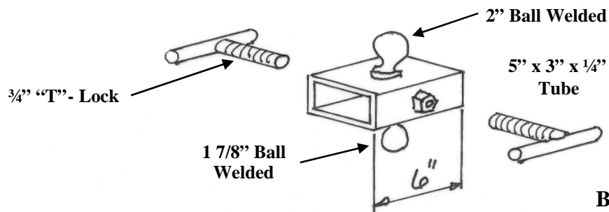
Benson Ball Hitch Model BBH - 1624 Wt. 56 lbs. List Price 360.00
